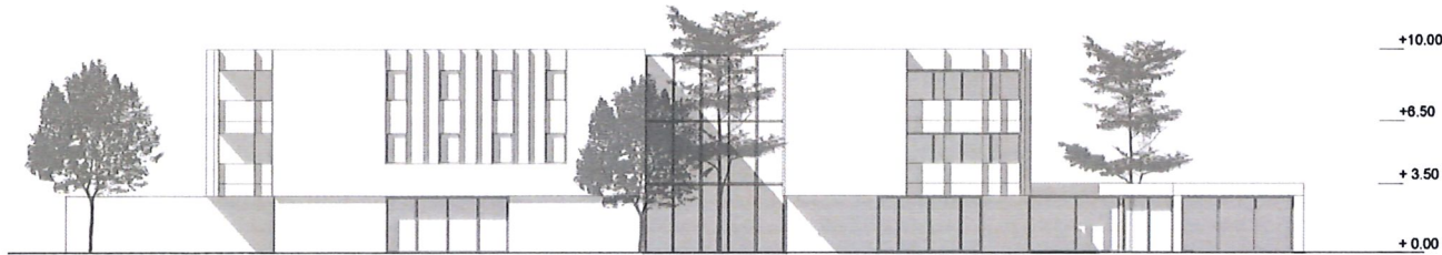
FACADE SUD
